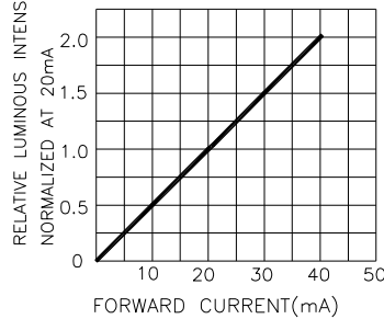
FORWARD CURRENT VS LUMINOUS INTENSITY
